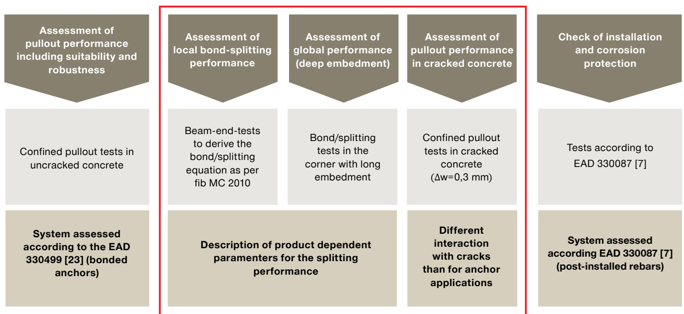
Fig. 3.7: Assessment of post-installed rebars according to EAD 332402 [10]
