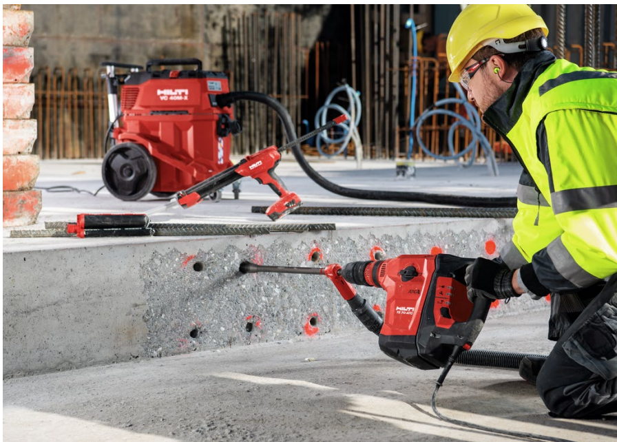
Fig. 9.16: Hilti SafeSet™ system – dust-free drilling of holes with hollow drill bits (HDB)
