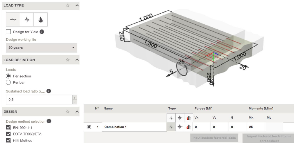
Fig. 8.7: Defining loads and load types in PROFIS
